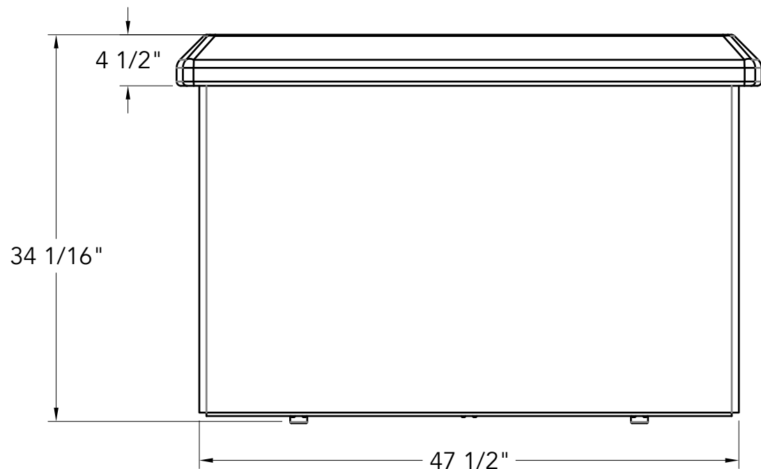
1 FRONT VIEW
