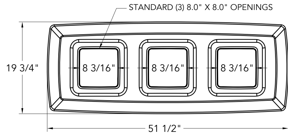
2 TOP VIEW
